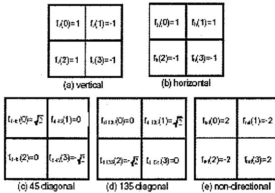
Figure 8 : Filter Coefficients For Edge Detection
