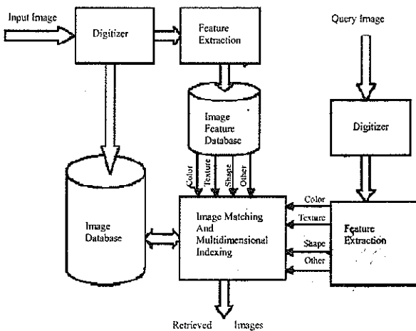
Figure 3 : General Scheme of Content Based Image Retrieval
